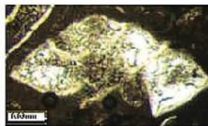
Globotruncanita conica
