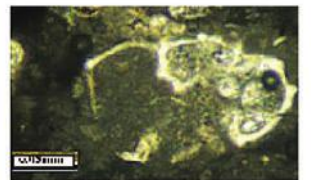
Globotruncana aegyptiaca
