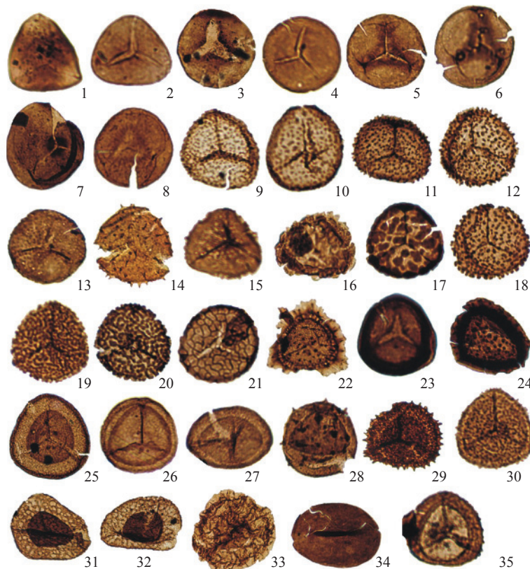
Fig. 1. Deltoidospora trivialis (Naumova) Braman & Hills, 1992. \times 1000 . Fig. 2. Leiotriletes inermis (Waltz) Ishchenko, 1952. \times 700 . Fig. 3. Punctatisporites stabilis Playford, 1962. \times 300 . Fig. 4. Punctatisporites sp. A. \times 800 . Figs. 5, 6. Retusotriletes planus Dolby & Neves, 1970. \times 600 . Fig. 7. Retusotriletes rotundus (Streel) Streel, 1967. \times 400 . Fig. 8. Retusotriletes rugulatus Riegel, 1973. \times 500 . Figs. 9, 10. Apiculatasporites sp. cf. A. perpusillus (Naumova ex Chibrikova) McGregor, 1973. \times 700 . Figs. 11, 12. Apiculatasporites brevidenticulatus (Chibrikova) McGregor & Camfield, 1982. \times 700 . Fig. 13. Cyclogranisporites sp. A. \times 700 . Fig. 14. Apiculatisporites sp. A. \times 500 . Fig. 15. Tricidarisporites sp. A. \times 900 . Fig. 16. Verrucosisporites sp. cf. V. scurrus (Naumova) McGregor & Camfield, 1982. \times 700 . Fig. 17. Verrucosisporites sp. A. \times 700 . Fig. 18. Raistrickia sp. A. \times 700 . Fig. 19. Convolutispora sp. A. \times 800 . Fig. 20. Convolutispora sp. B. \times 700 . Fig. 21. Dictyotriletes australis de Jersey, 1966. \times 500 . Fig. 22. Vallatisporites hystricosus (Winslow) Byvscheva, 1985. \times 500 . Fig. 23. Densosporites? cassiformis (Chibrikova) Arkhangelskaya, 1985. \times 700 . Fig. 24. Densosporites spitsbergensis Playford, 1963. \times 500 . Fig. 25. Concentricosisporites sagittarius Rodriguez, 1983. \times 300 . Figs. 26, 27. Geminospora lemurata Balme emend Playford, 1983. \times 700 . Fig. 28. Grandispora cornuta Higgs, 1975. \times 500 . Fig. 29. Grandispora famenensis (Naumova) Streel var minuta Nekriata, 1974. \times 500 . Fig. 30. Grandispora sp. A. \times 800 . Figs. 31, 32. Retispora lepidophyta (Kedo) Playford, 1976. 31. \times 500 . 32. \times 300 . Fig. 33. Rugospora sp. A. \times 400 . Fig. 34. Laevigatisporites sp. A. \times 400 . Fig. 35. Coptospora sp. \times 700 .
