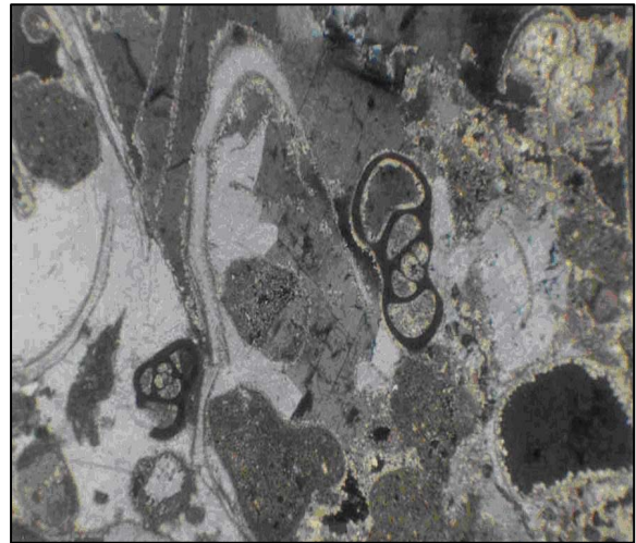
Fig.11- Dolomitized bioclastic packstone porosity: mouldic
