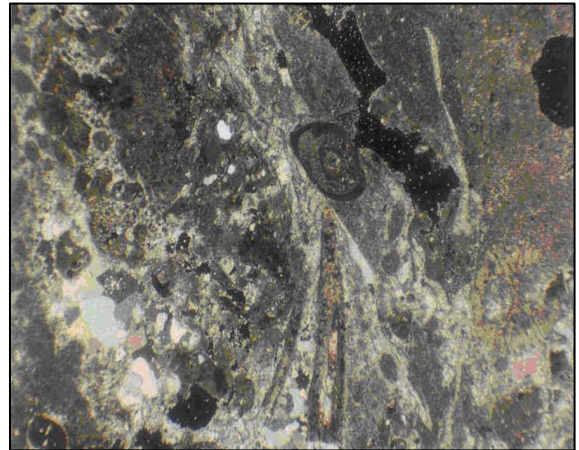
Fig.9- Bioclastic packstone porosity (vugg & mouldic)
