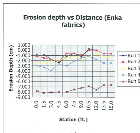
Figure 6- Erosion depths versus distance for Enka Fabrics
