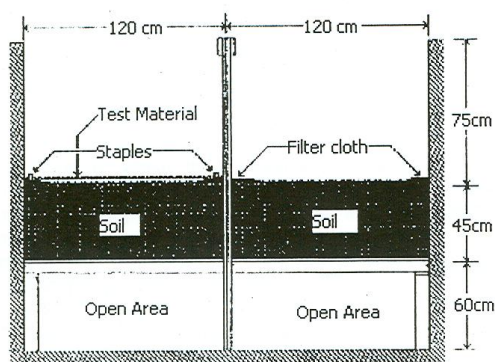
Figure 2-Flume cross section showing anchoring of materials and side curtains
