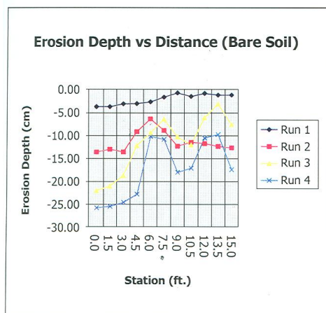
Figure5- Erosion depth versus distance for bare soil
