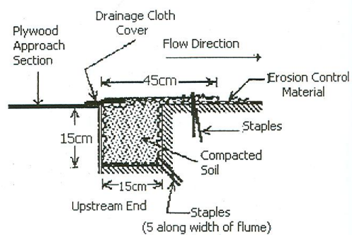
Figure 3- Head trench for anchoring test materials.
