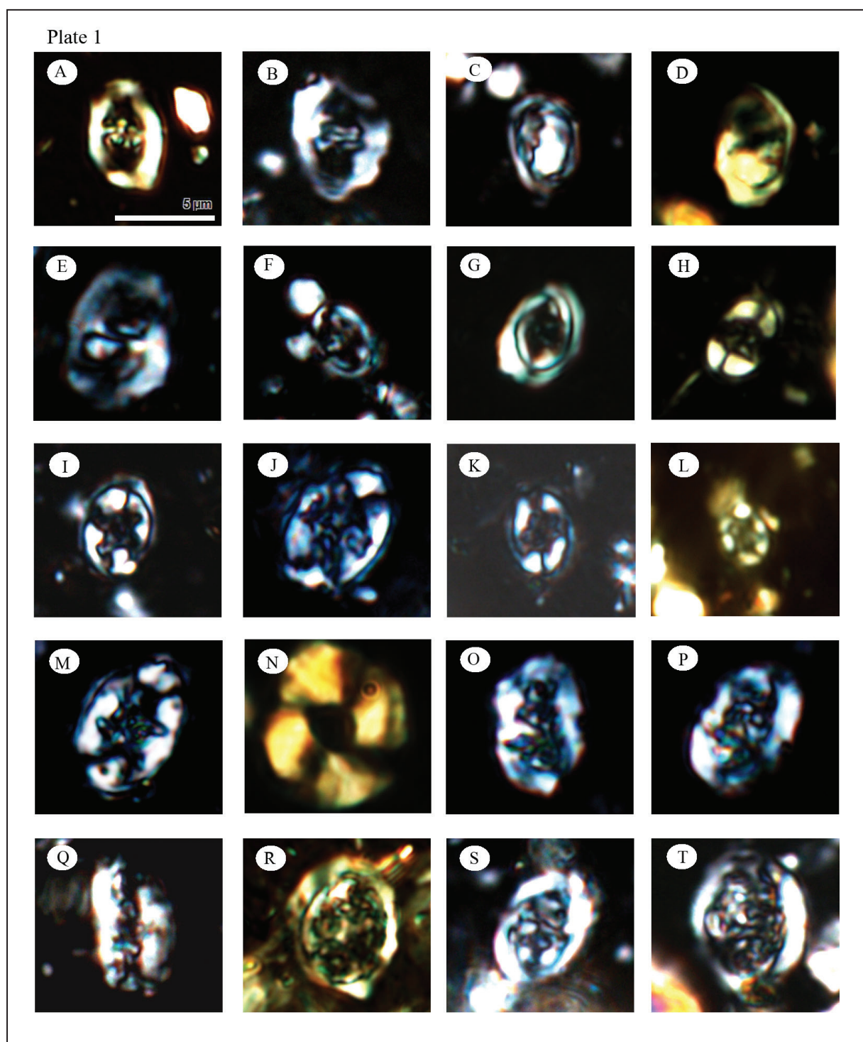
Plate 1- Cross Polarized light (XPL) of calcareous nannofossil pictures from early Cretaceous of Nimbolook section. (MN= Nimbolook). Scale bar for all pictures: 5 \mu m.
