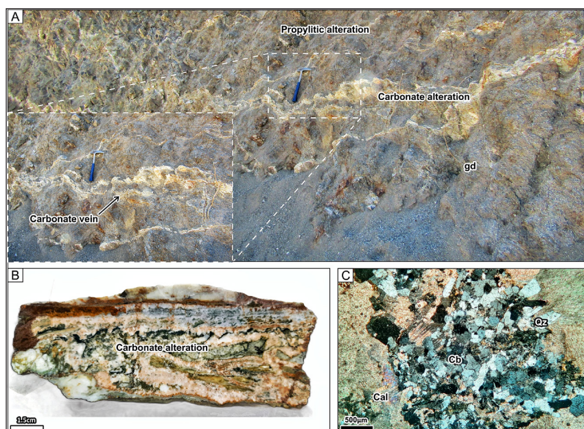
Figure 11- A) View of the occurrence of carbonatic and propylitic alteration in a granodiorite body; B) Hand specimen image of the carbonatic alteration; C) Microscopic image showing the association of quartz, calcite (Cal), and other carbonate minerals (Cb) that formed during carbonatic alteration along with quartz (Qz).
