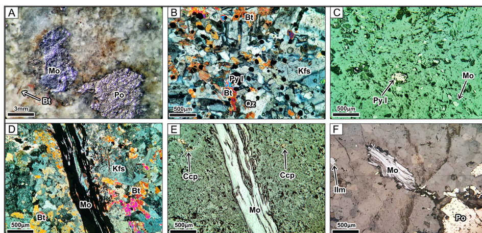
Figure 15- A) Photograph illustrating the spatial association of molybdenite (Mo), pyrrhotite (Po), and fine-grained biotite crystals (Bo); B and C) photomicrographs showing quartz (Qtz), K-feldspar (Kfs), and biotite (Bt), in which first-generation molybdenite (Mo I) and first-generation pyrite (Py I) occur as disseminated grains in close paragenetic association with these phases.; D and E) Occurrence of K-feldspar (Kfs) and biotite (Bt) within the altered quartz monzonite, hosting second-generation molybdenite (Mo II) with a veinlet-style texture accompanied by disseminated chalcopyrite (Ccp); F) Photomicrograph showing the intergrowth of second-generation molybdenite (Mo II), ilmenite (Ilm), and pyrrhotite (Po).
