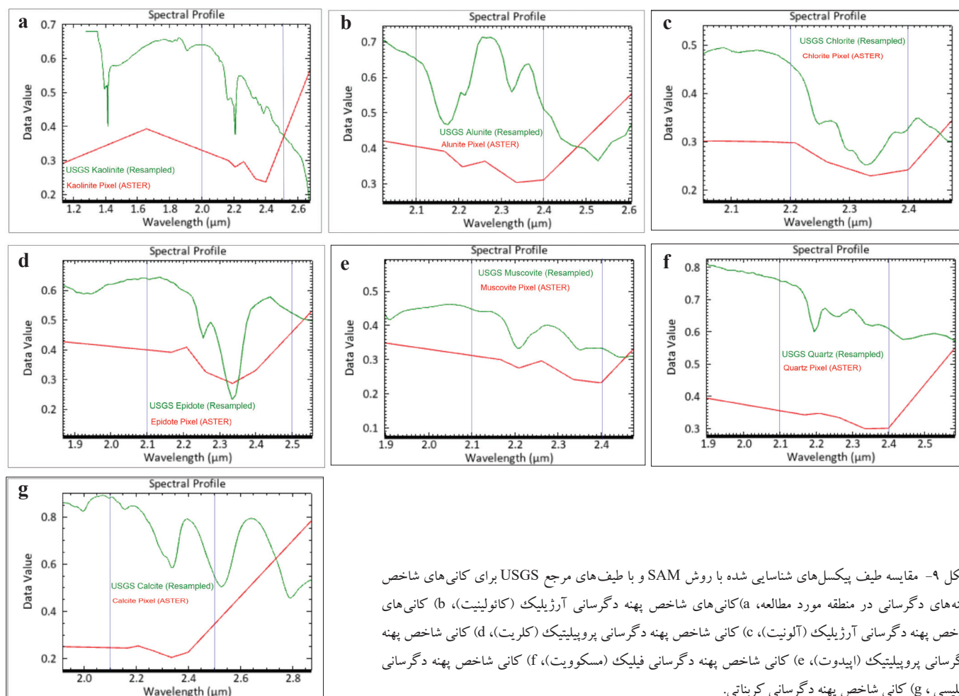
Figure 9. Comparison of the spectra of pixels identified using the SAM method with the USGS reference spectra for the indicator minerals of the alteration zones in the study area: a) indicator minerals of the argillic alteration zone (kaolinite), b) indicator minerals of the argillic alteration zone (alunite), c) indicator mineral of the propylitic alteration zone (chlorite), d) indicator mineral of the propylitic alteration zone (epidote), e) indicator mineral of the phyllic alteration zone (muscovite), f) indicator mineral of the silicic alteration zone, and g) indicator mineral of the carbonate alteration zone.
